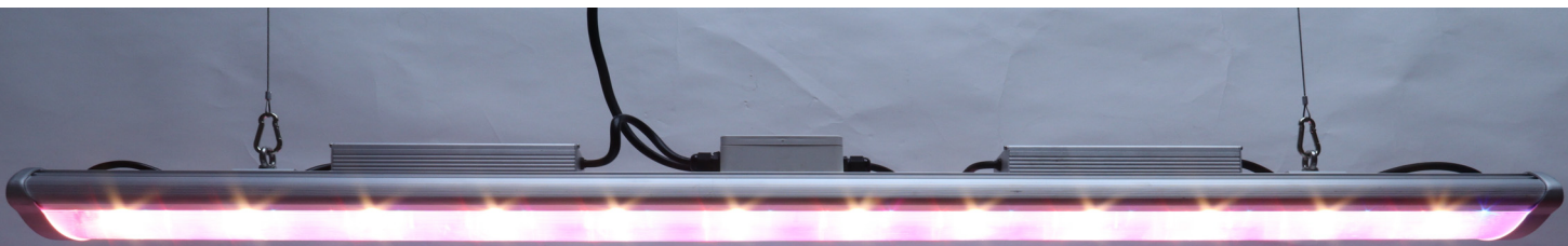
OPTIONAL MOUNTING BRACKETS (DOUBLE LIGHTS IN A LINE)
